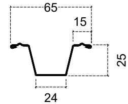
25mm BATTEN (0.42 bmt)
