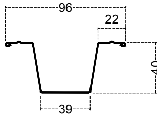
40mm BATTEN (0.55 bmt) (0.75 bmt)
